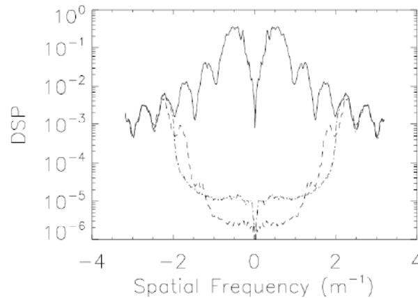
Figure 11. Static coronagraphic PSF profiles before (solid) and after correction by a DM (dashed: least-squares fitting of influence functions, dashed-dotted: Fourier filtering used for EPICS analysis).
