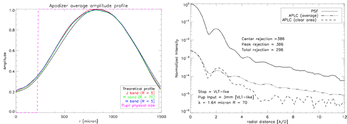
Figure 6. Laboratory measurements of the APLC. Left: Measured profile of the binary apodizer mask, Right: Coronagraphic PSF profile. The azimuthally averaged rejection suffers from a mismatch between telescope spider arms and the Lyot stop.
