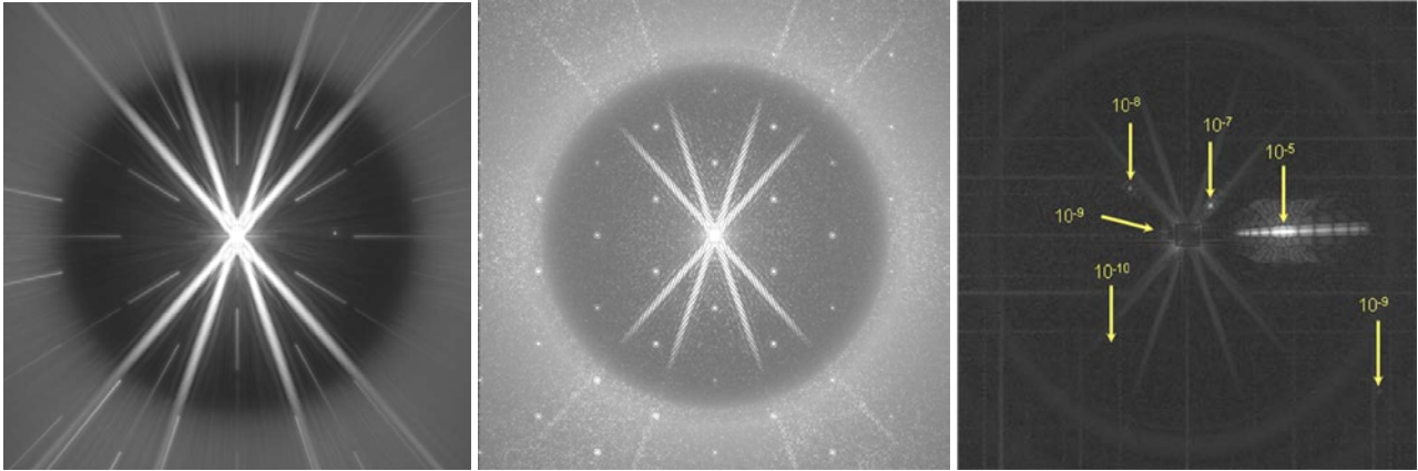
Figure 9. IFS data reduction with static aberrations only and perfect coronagraph. Left: Wide – band image showing speckle elongation. Middle: Spatially rescaled version of image on the left. Speckles are point-like, the hidden planets are elongated. Right: SD subtraction of residual PSF, the contrast is efficiently enhanced.
