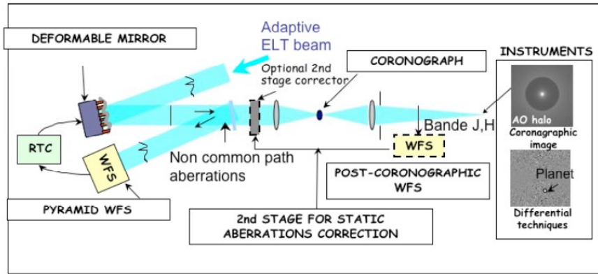
Figure 4. Basic concept and main components of EPICS
