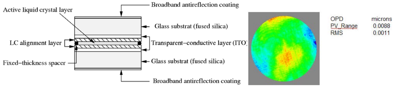
Figure 8. Left: Cross section of an FLC modulator from BNS. Right: Measured differential wave front error of 1.1 nm after removal of tip-tilt.
