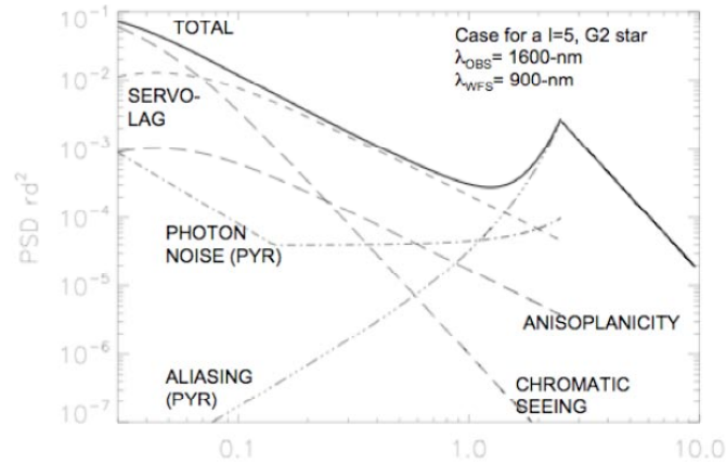
Figure 10. Analytical profile of the coronagraphic PSF provided by the EPICS XAO concept (modulated PWS, actuator spacing 0.2-m, framerate 3kHz). The temporal error (servo-lag) dominates the residual WFE.
