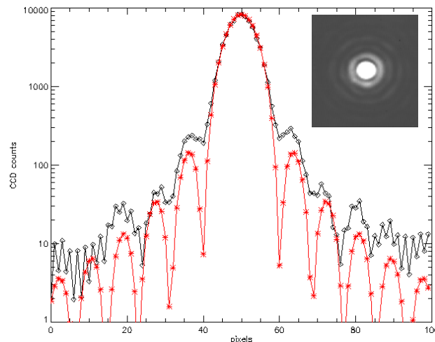
Figure 5. HOT XAO images obtained in H-band (from Esposito et al., proceedings of SPIE 7015, 2008).
