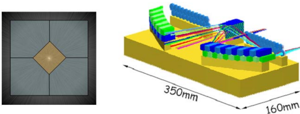
Figure 7 Left: Possible split of the EPICS lenslet-based IFS field of view superimposed to a simulated monochromatic image. The central orange square area (0.6 arcsec side) is most important for exoplanet science. Right: 3-D design of the Image Slicer prototype.
